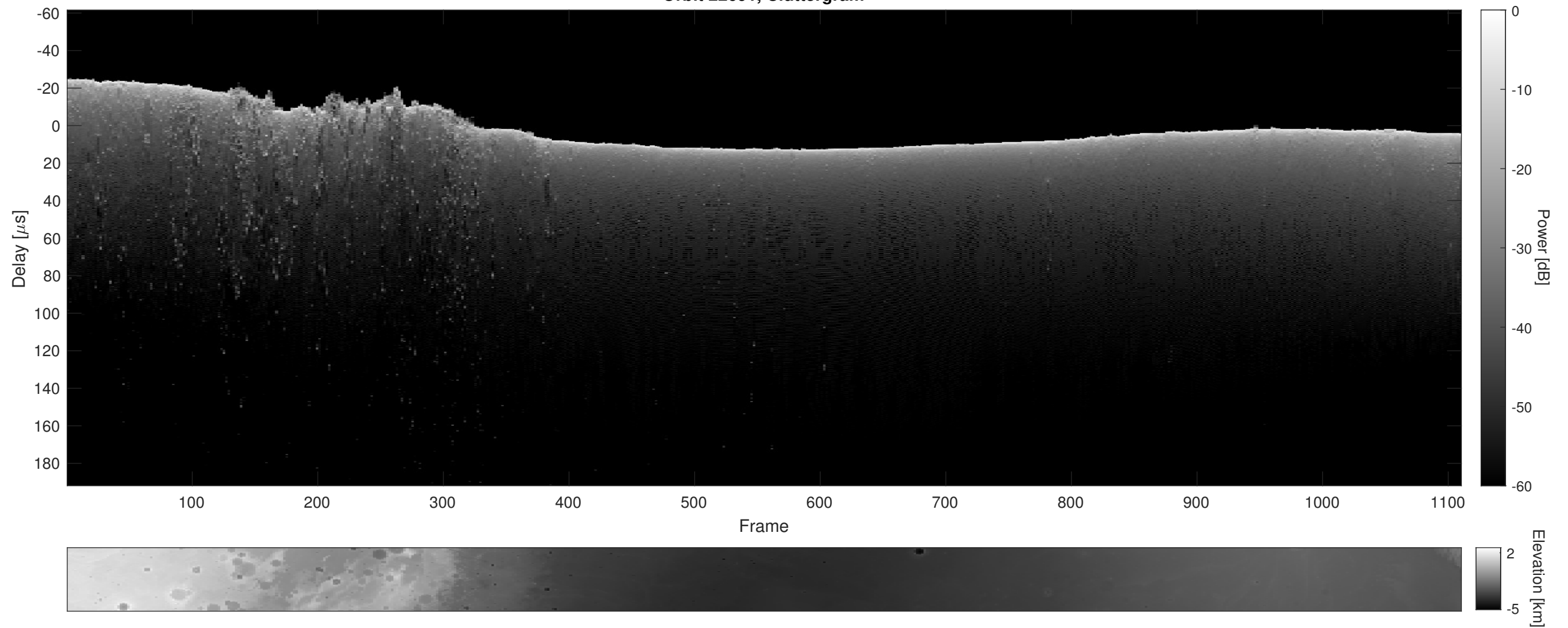
Orbit 22691, Cluttergram
