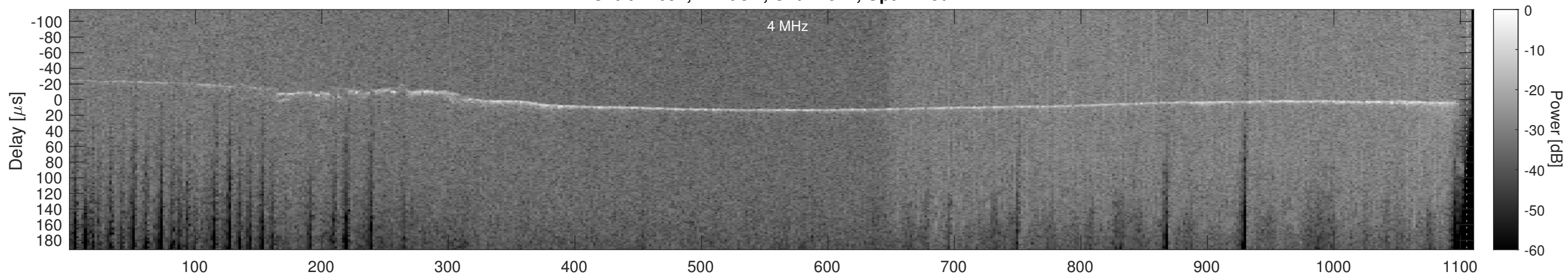
Orbit 22691, Cluttergram
