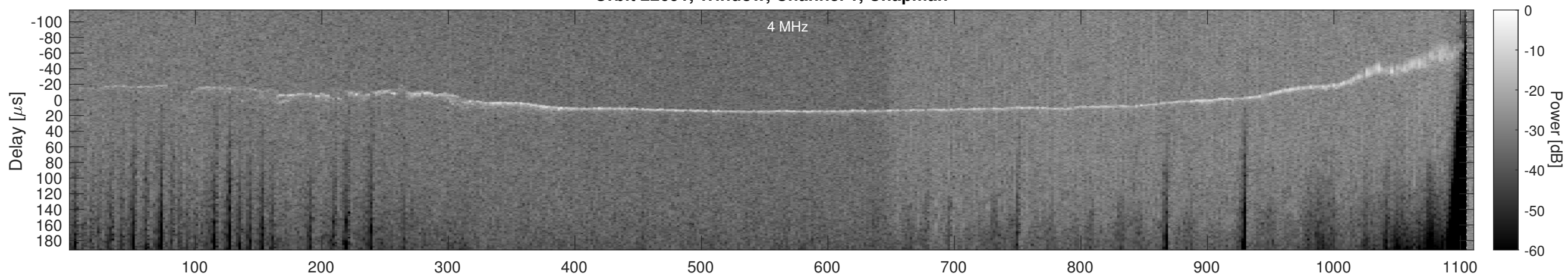
Orbit 22691, Window, Channel 1, Optimized
