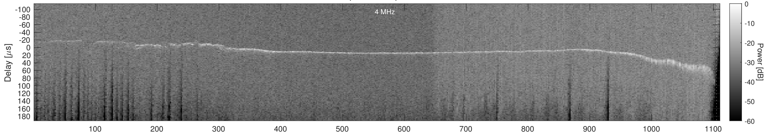
Orbit 22691, Window, Channel 1, Chapman
