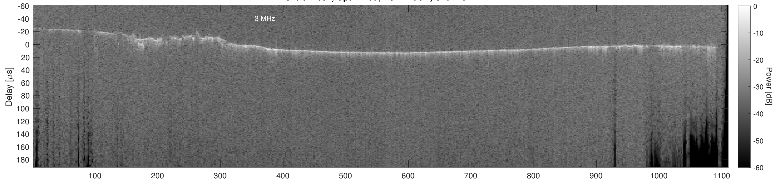
Orbit 22691, Cluttergram
