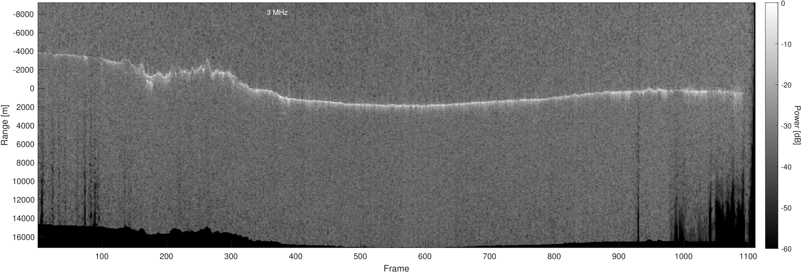
Orbit 22691, Optimized, No Window, Depth-Corrected, Channel 2
