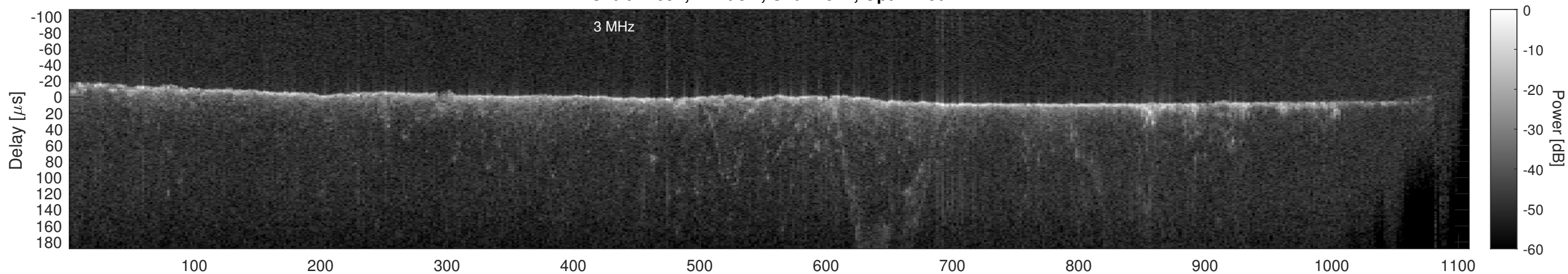
Orbit 22692, Cluttergram
