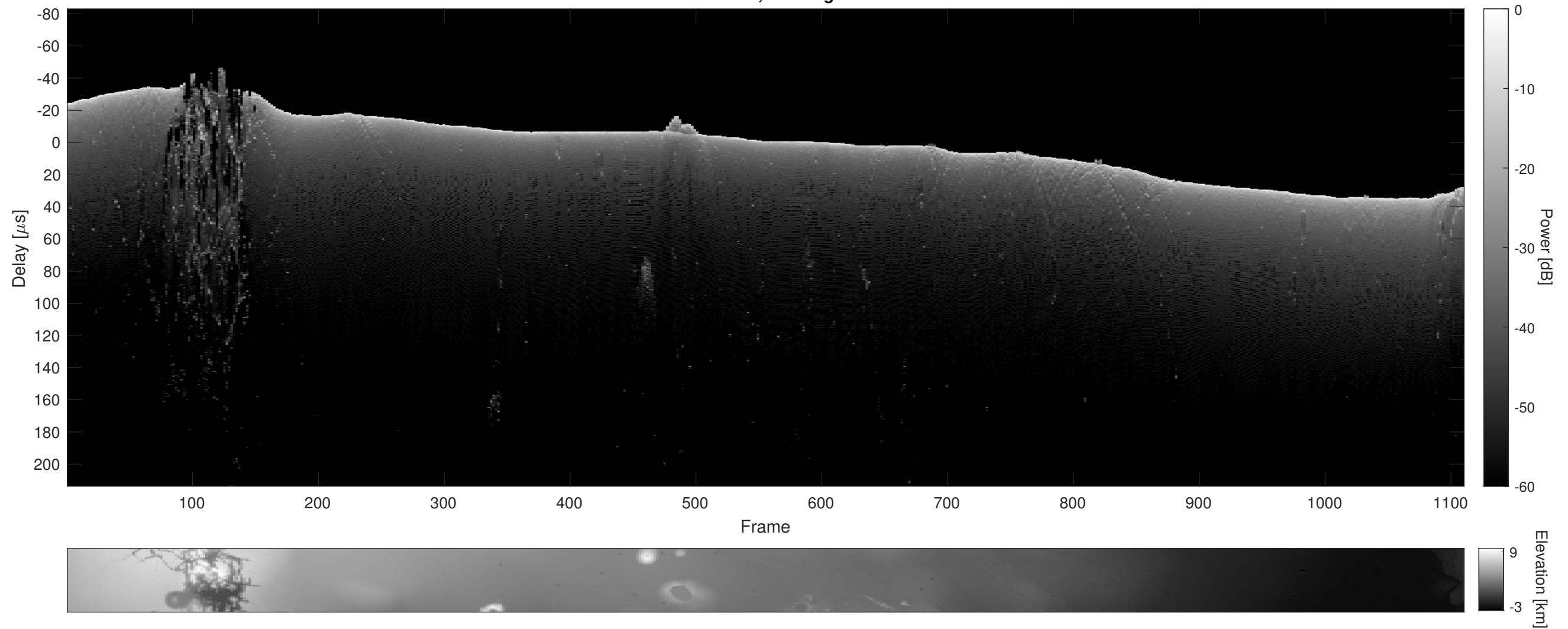
Orbit 22693, Cluttergram
