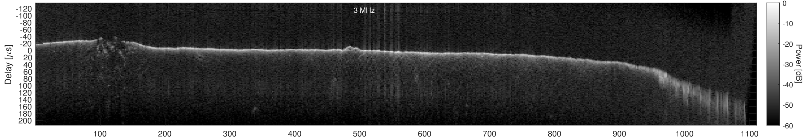
Orbit 22693, Window, Channel 2, Chapman
