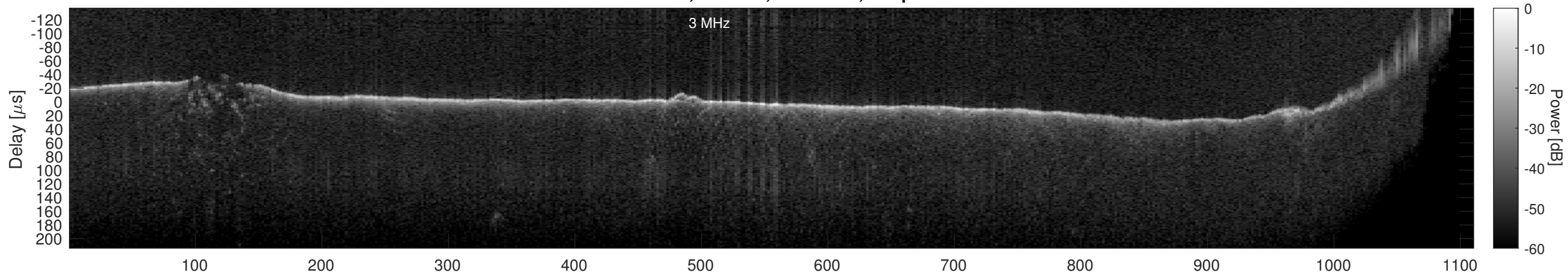
Orbit 22693, Window, Channel 2, Optimized
