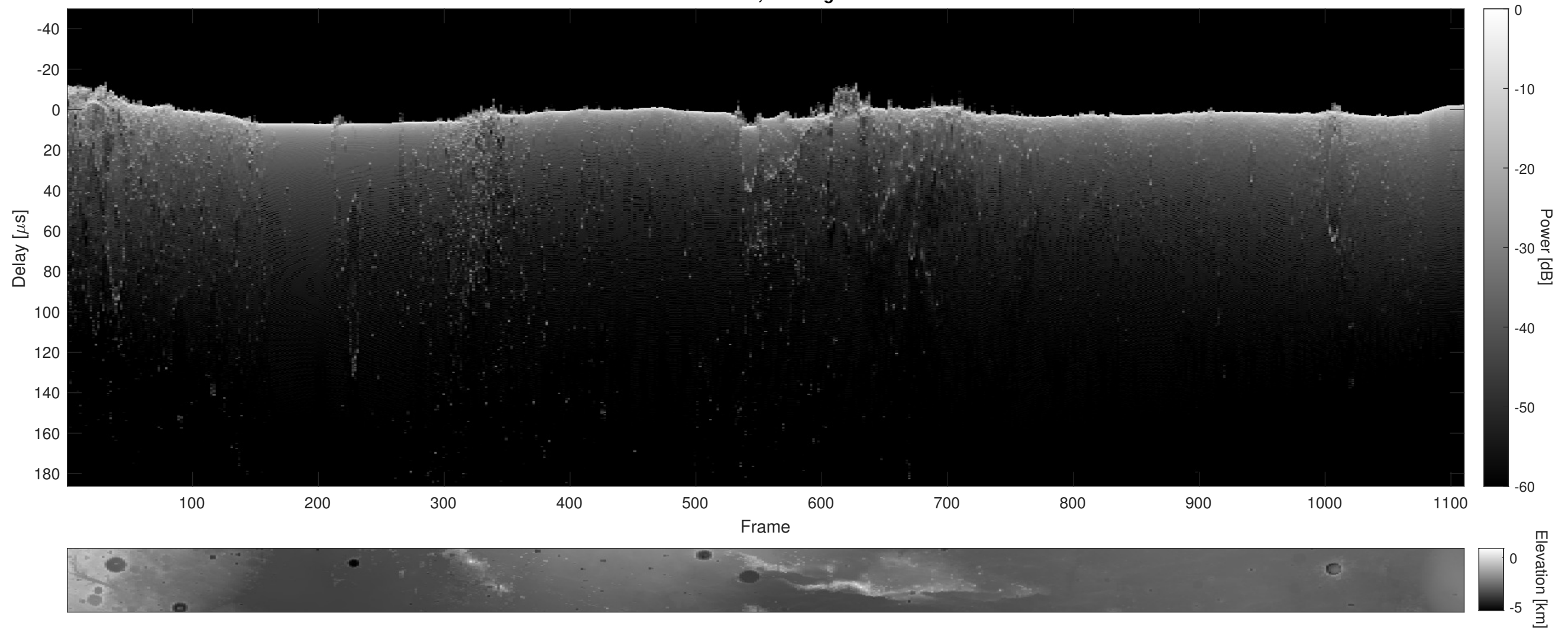
Orbit 22694, Cluttergram
