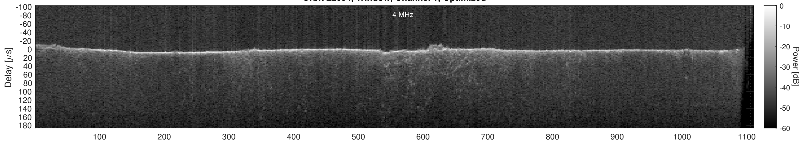
Orbit 22694, Cluttergram
