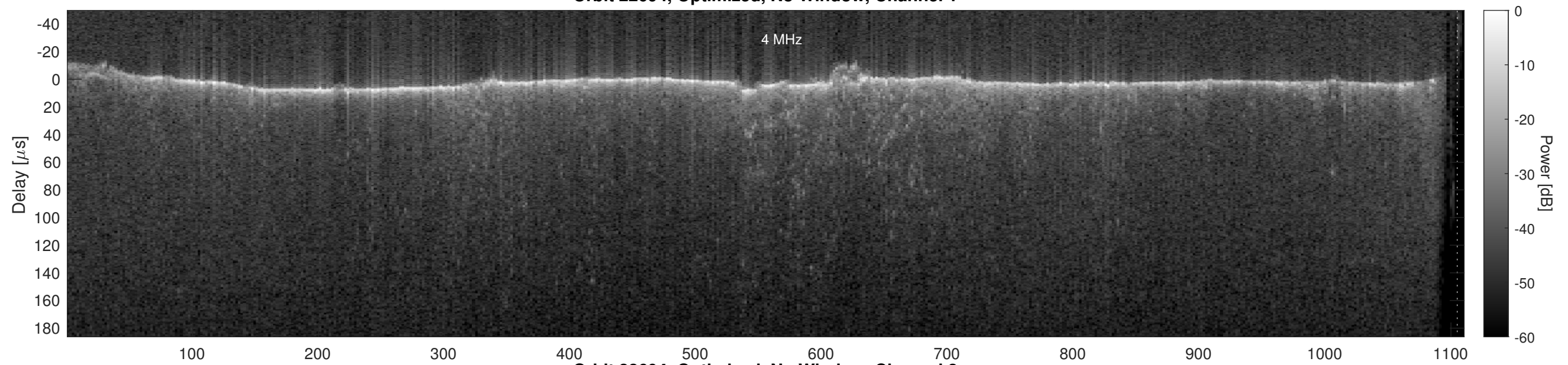
Orbit 22694, Optimized, No Window, Channel 2
