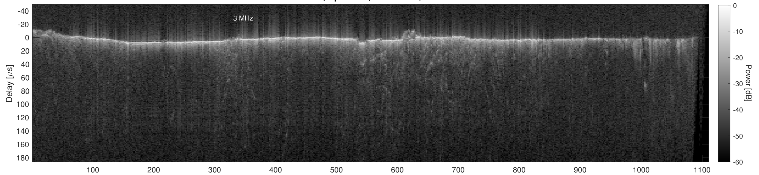
Orbit 22694, Cluttergram
