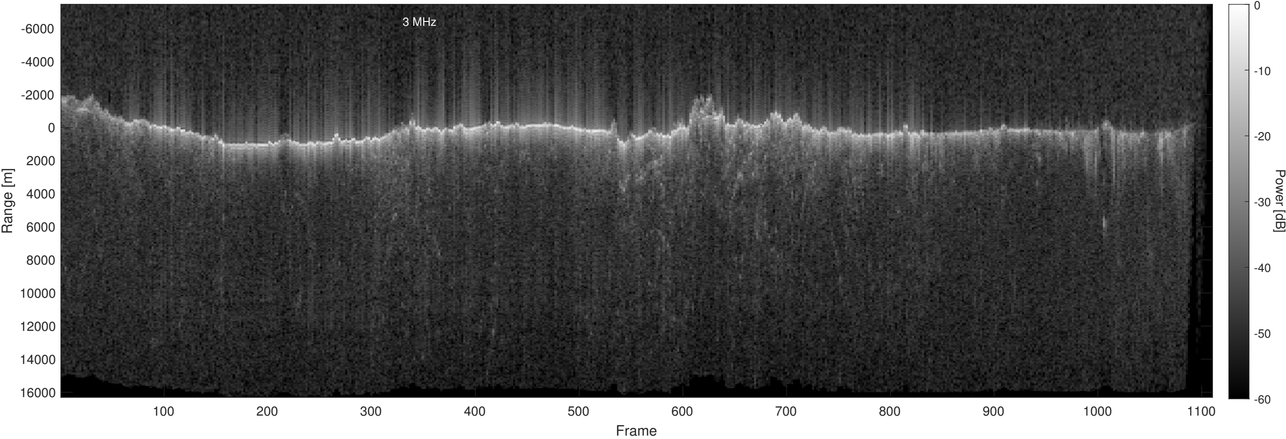
Orbit 22694, Optimized, No Window, Depth-Corrected, Channel 2
