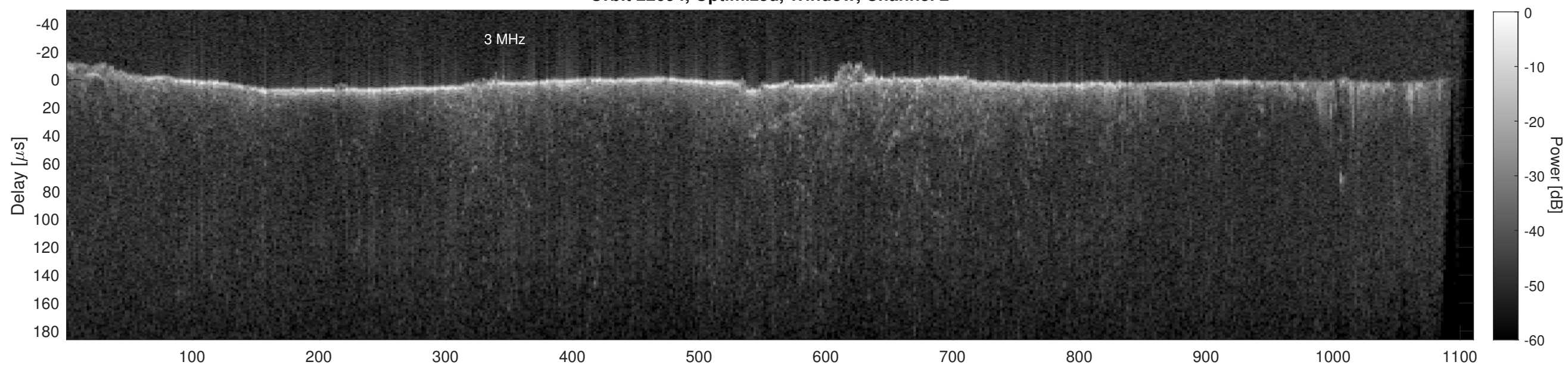
Orbit 22694, Cluttergram
