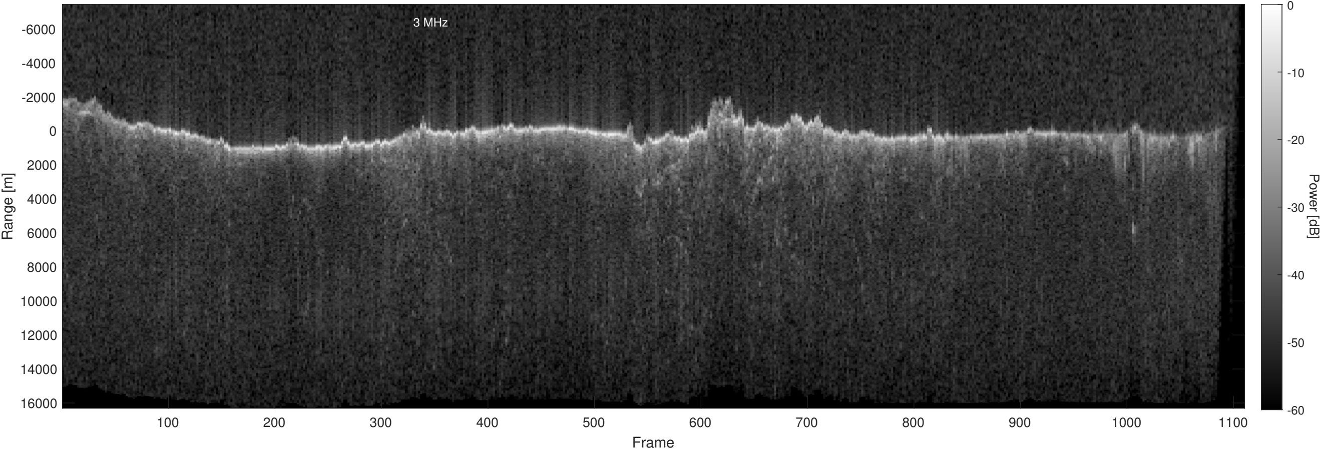
Orbit 22694, Optimized, Window, Depth-Corrected, Channel 2
