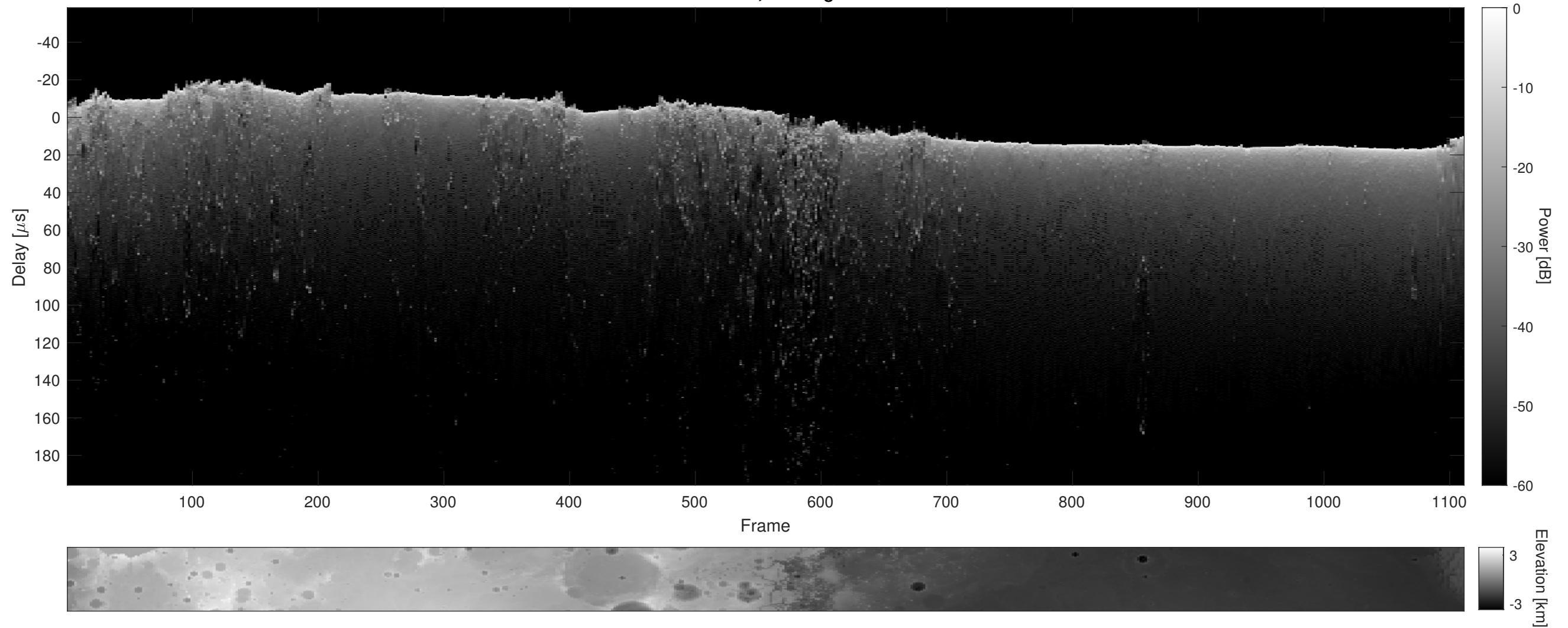
Orbit 22695, Cluttergram
