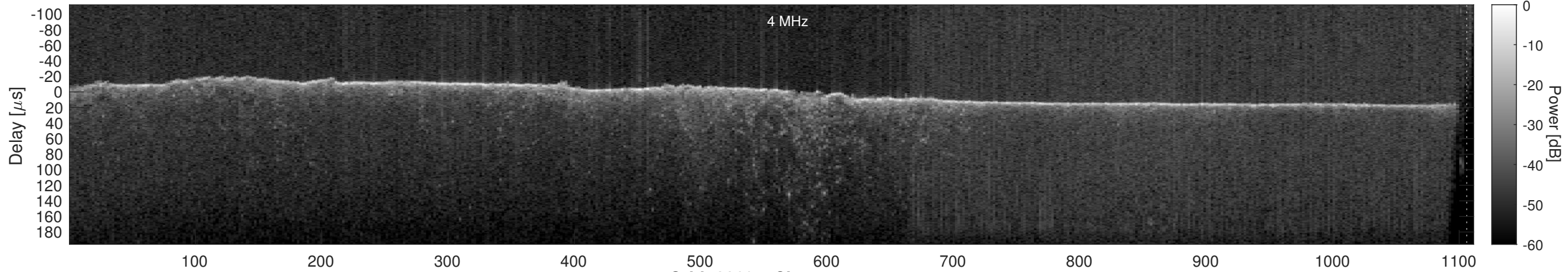
Orbit 22695, Cluttergram
