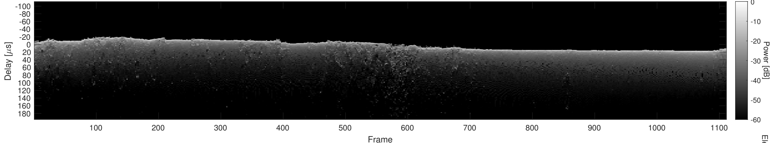
Orbit 22695, Cluttergram
