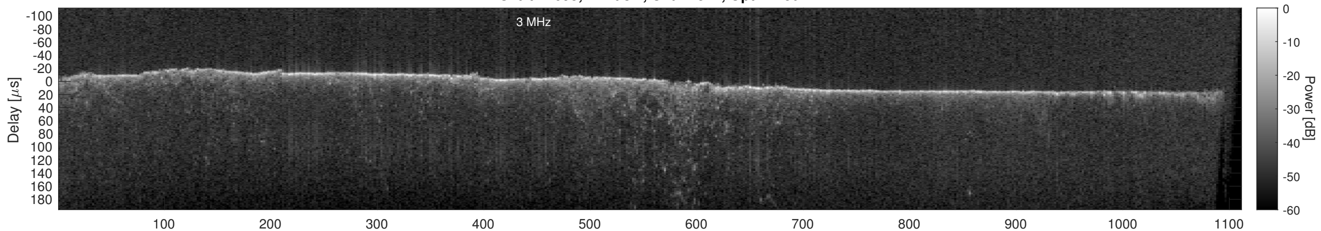
Orbit 22695, Cluttergram
