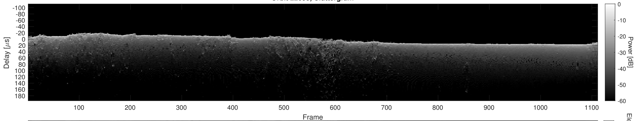
Orbit 22695, Cluttergram
