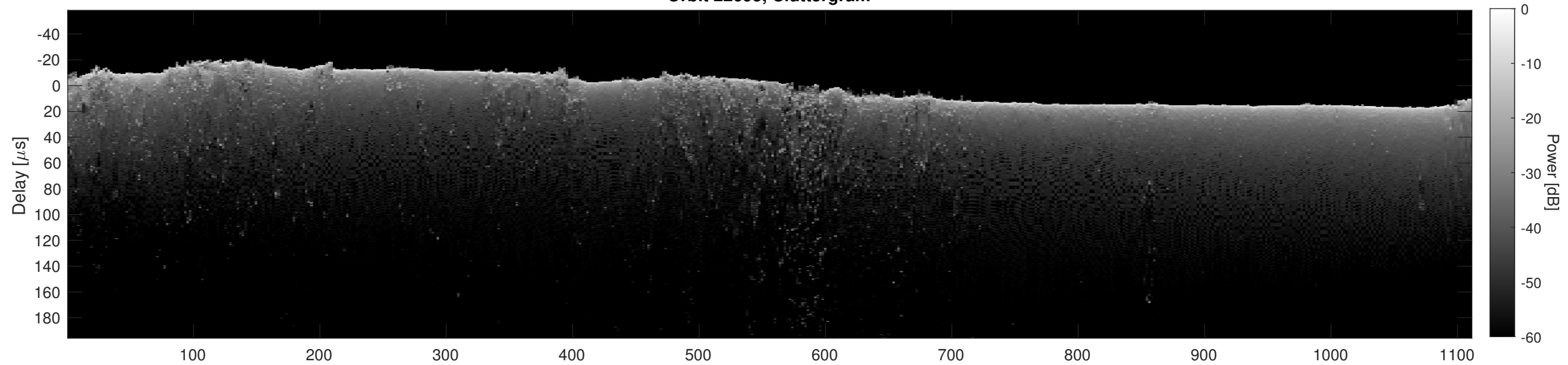
Orbit 22695, Cluttergram
