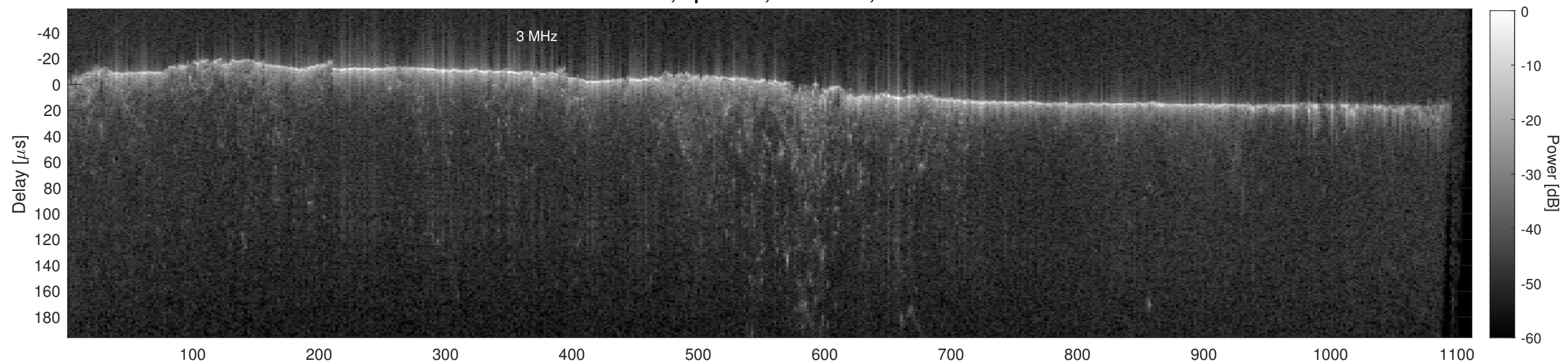
Orbit 22695, Cluttergram
