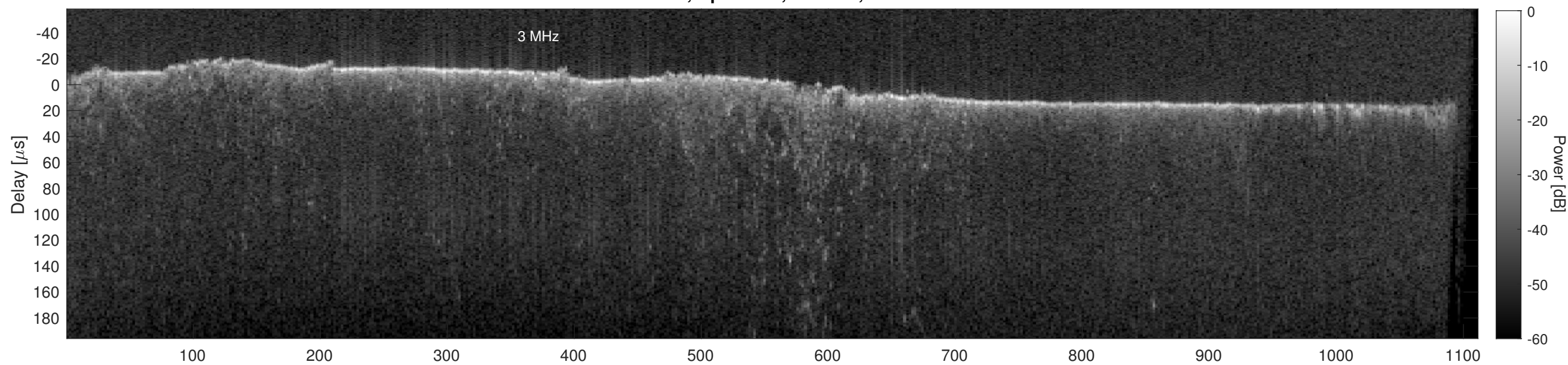
Orbit 22695, Cluttergram
