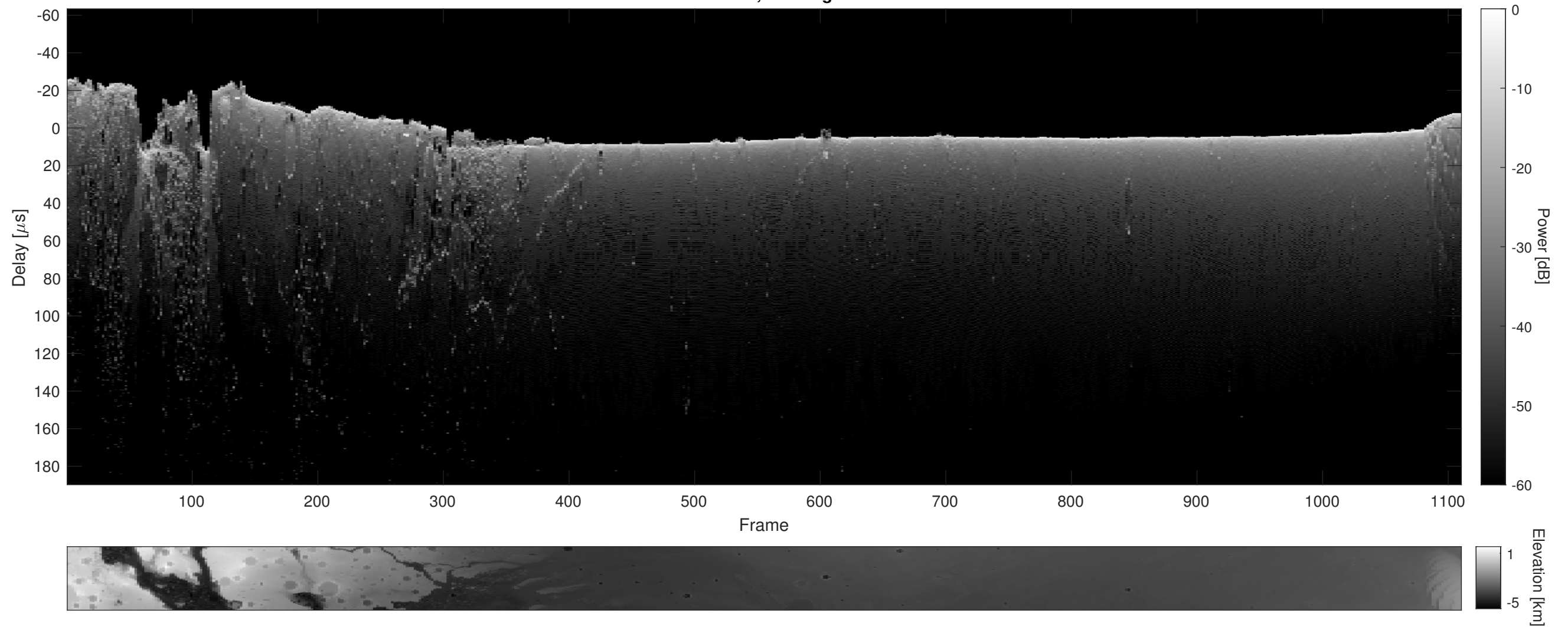
Orbit 22696, Cluttergram
