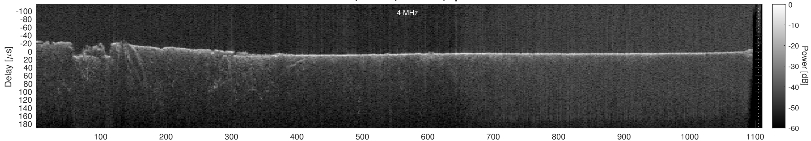
Orbit 22696, Cluttergram
