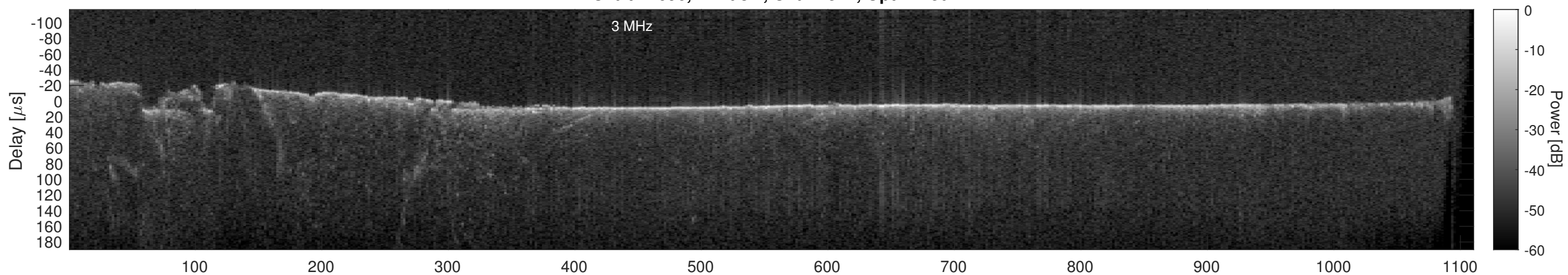
Orbit 22696, Cluttergram
