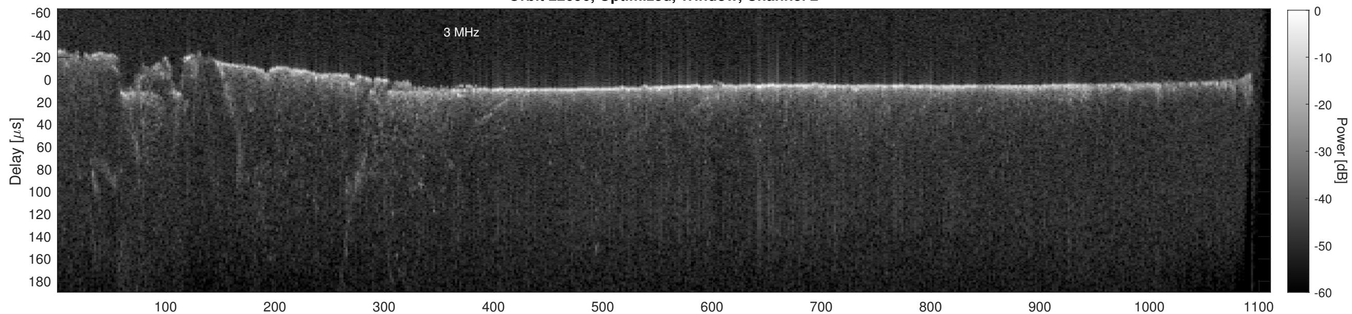
Orbit 22696, Cluttergram
