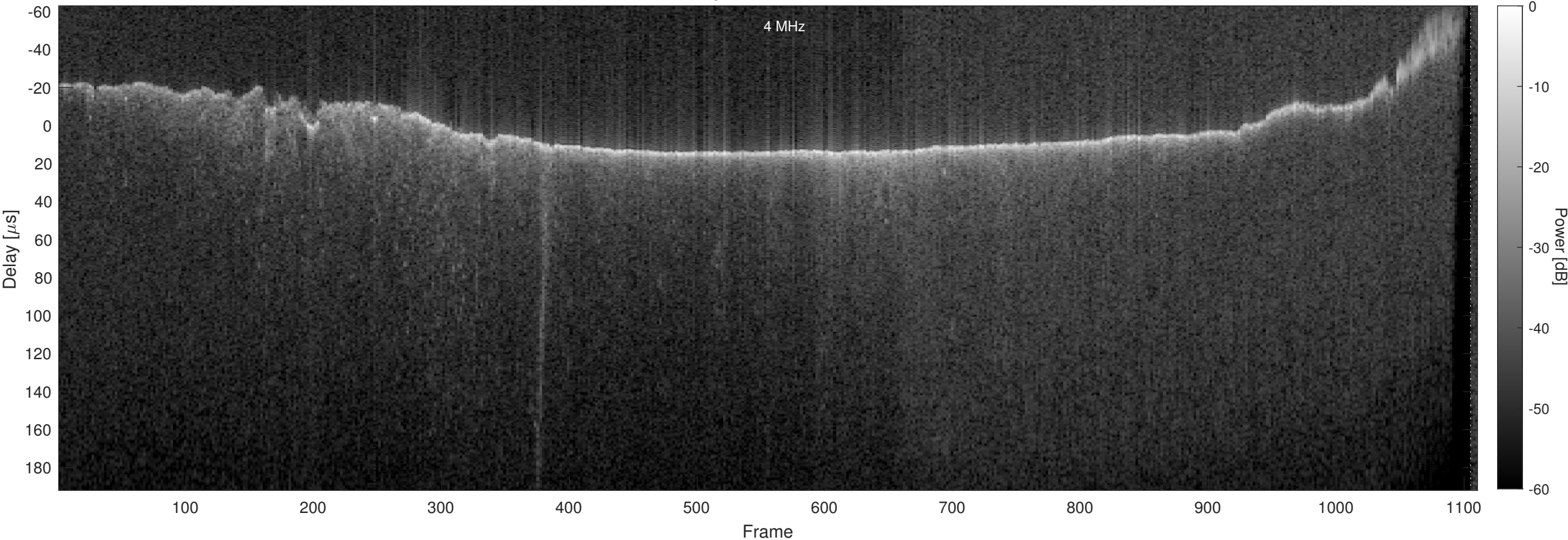
Orbit 22698, Chapman, No Window, Channel 2
