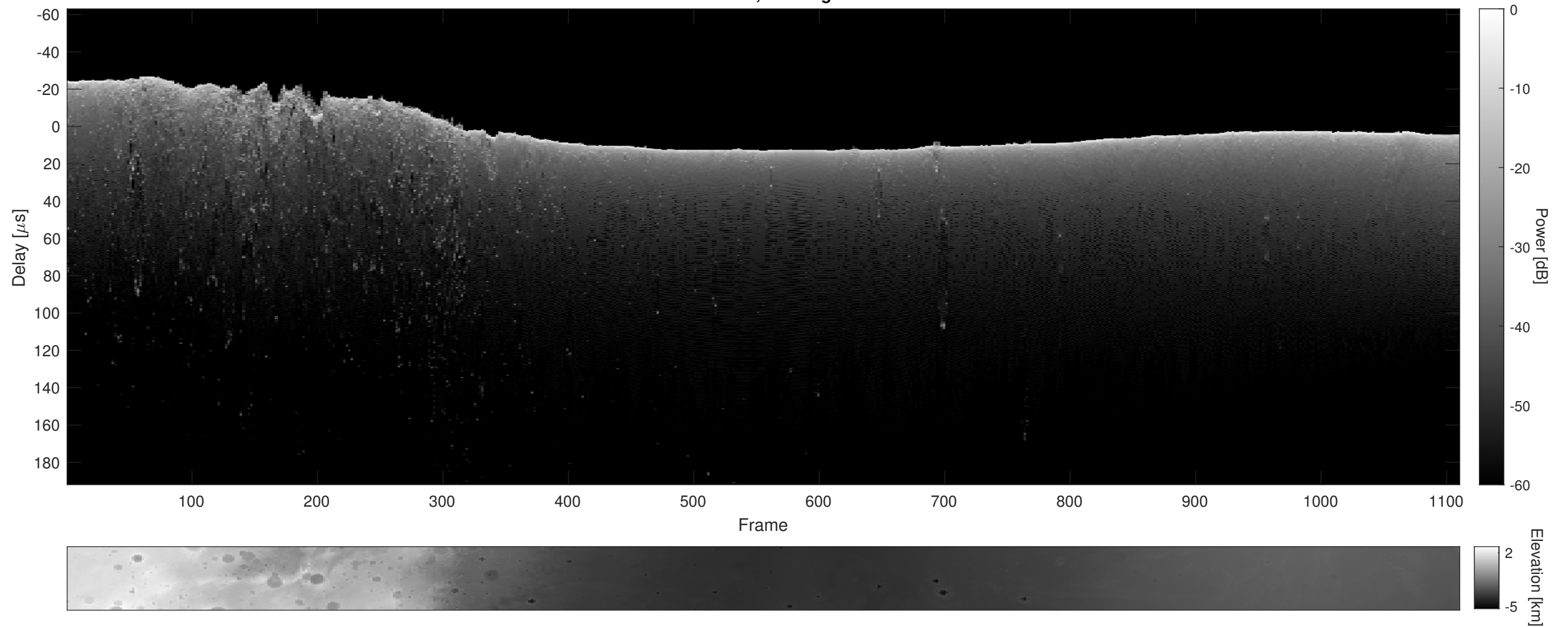
Orbit 22698, Cluttergram
