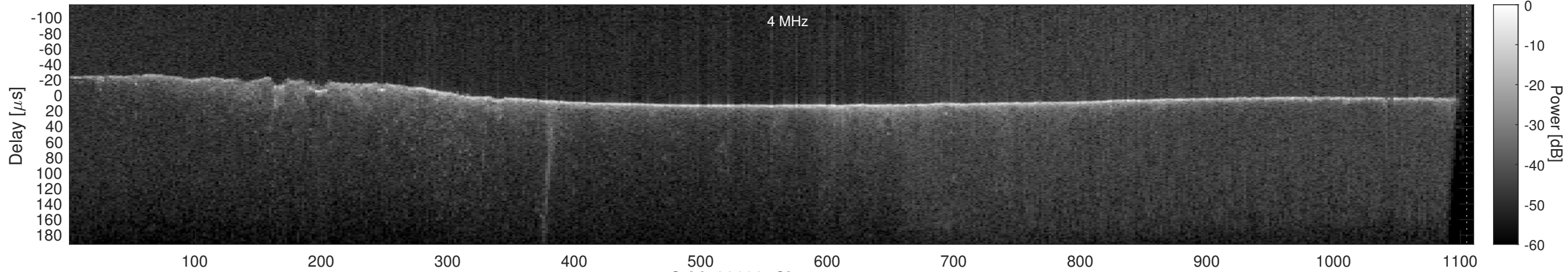
Orbit 22698, Cluttergram
