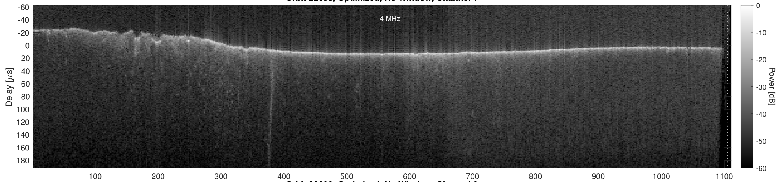
Orbit 22698, Optimized, No Window, Channel 2
