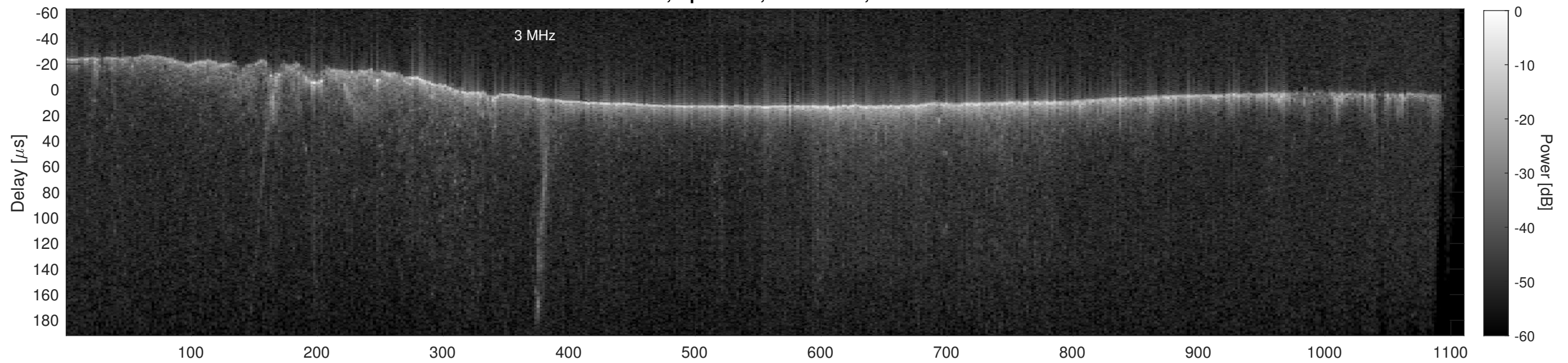
Orbit 22698, Cluttergram
