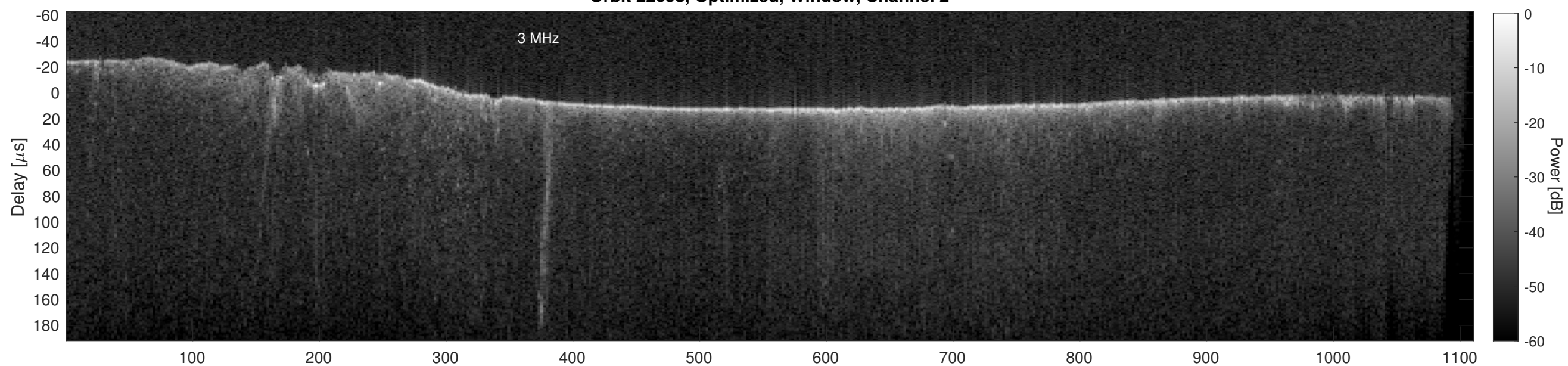
Orbit 22698, Cluttergram
