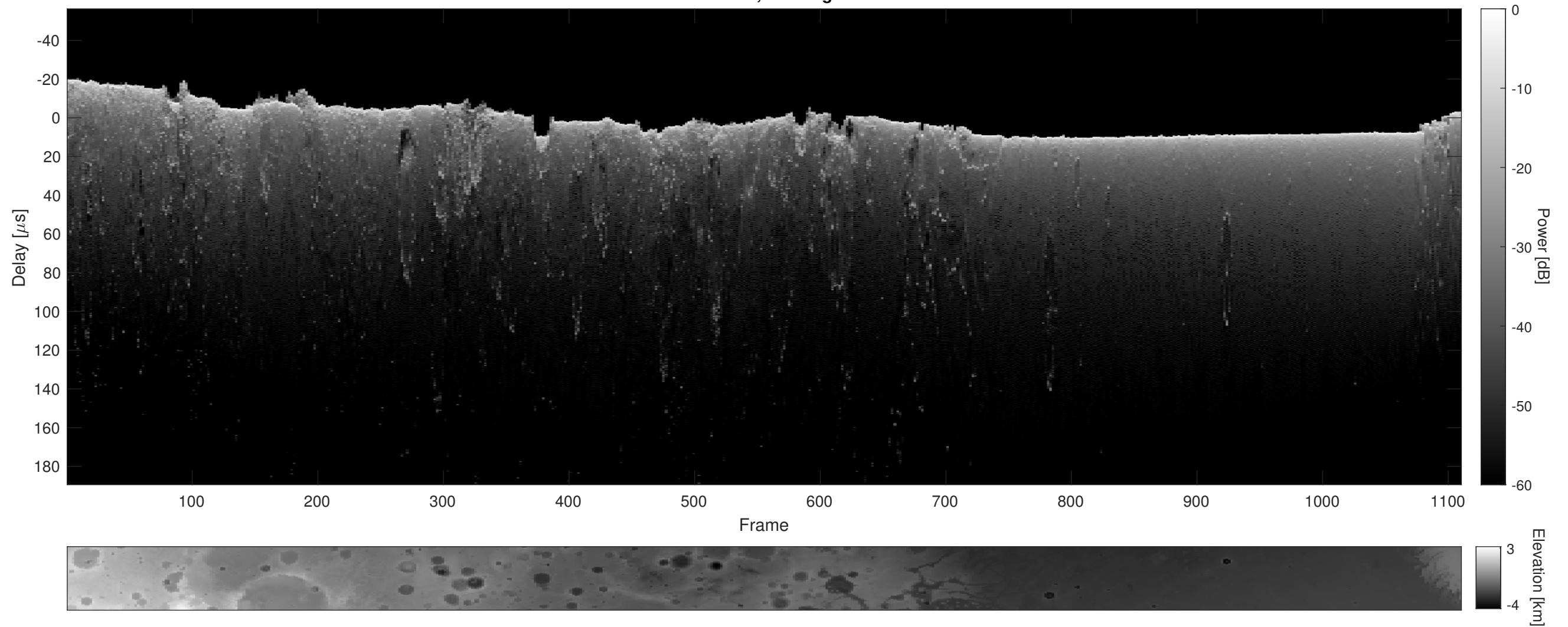
Orbit 22699, Cluttergram
