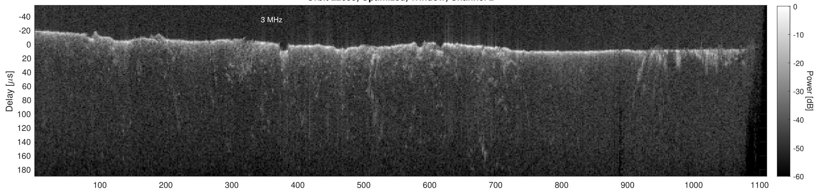
Orbit 22699, Cluttergram
