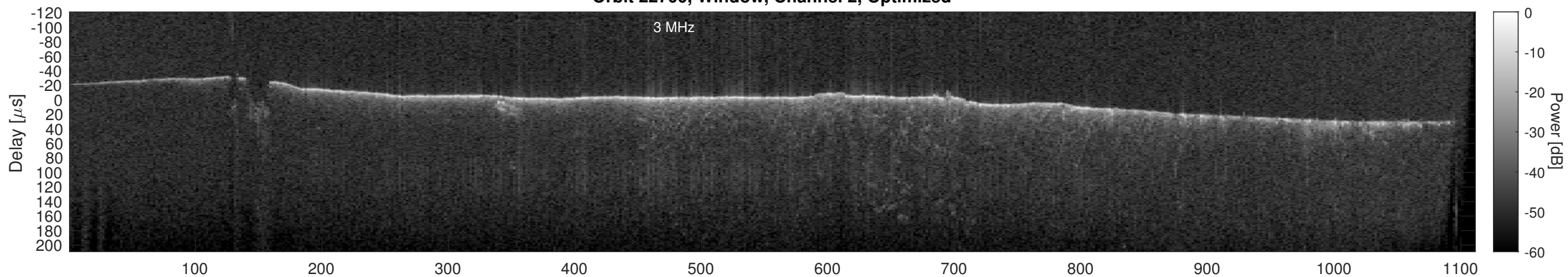
Orbit 22700, Cluttergram
