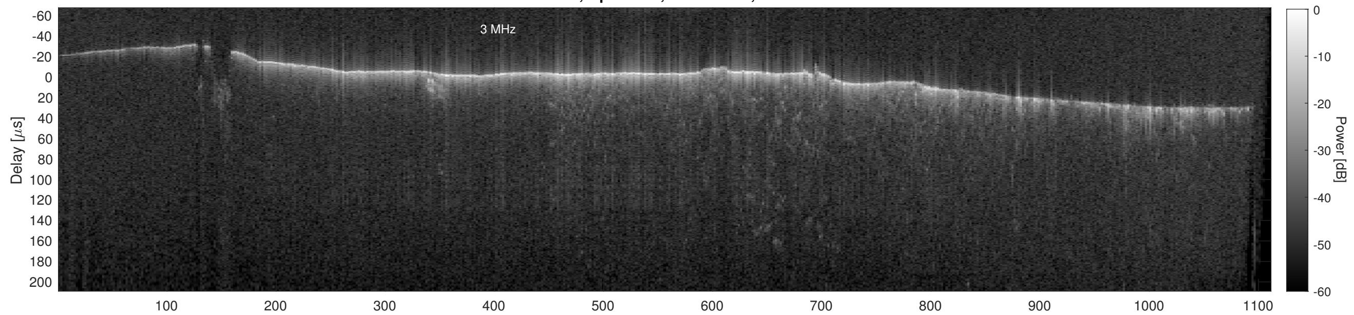
Orbit 22700, Cluttergram
