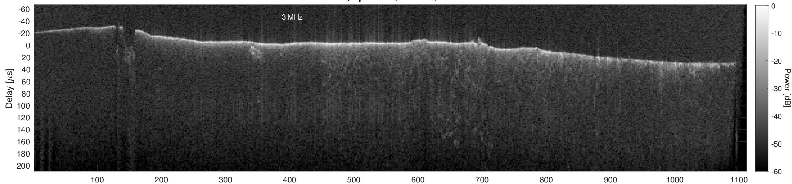
Orbit 22700, Cluttergram
