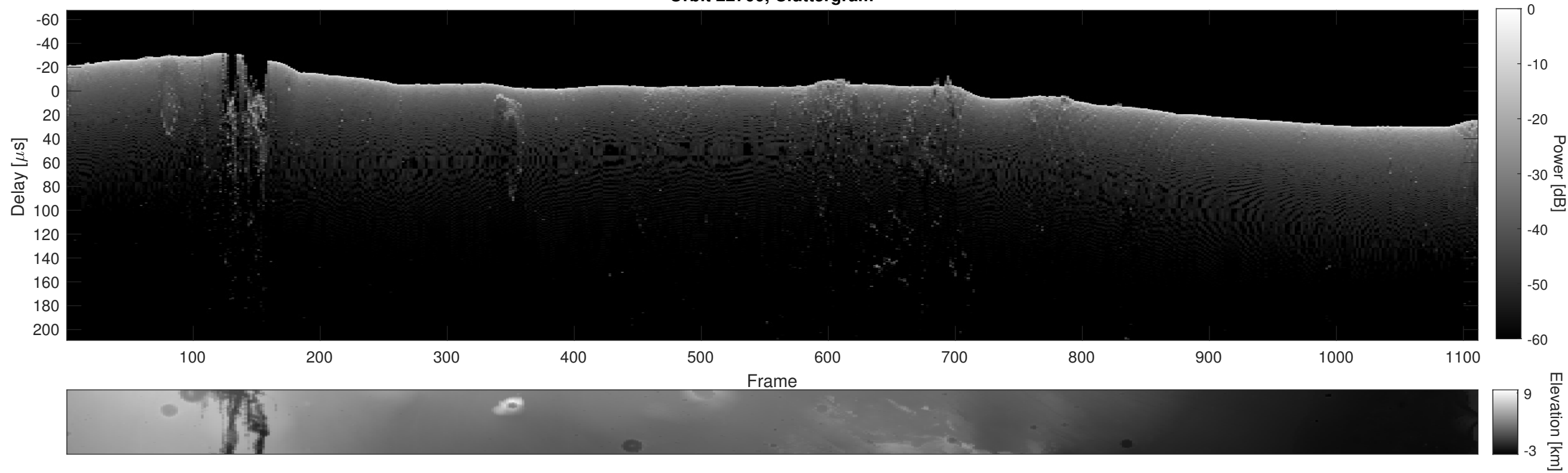
Orbit 22700, Cluttergram
