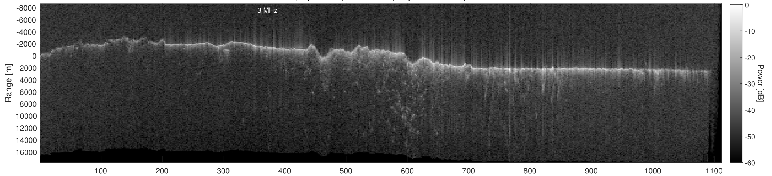
Orbit 22702, Depth-Corrected Cluttergram
