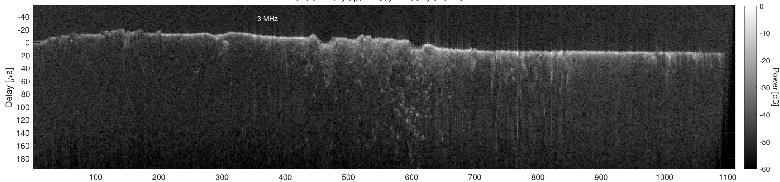
Orbit 22702, Cluttergram
