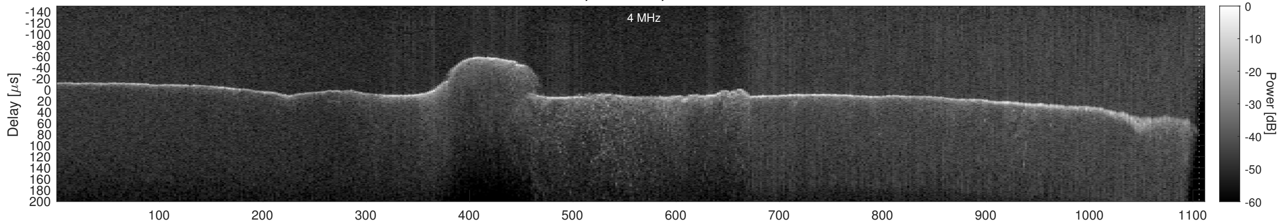
Orbit 22704, Window, Channel 1, Chapman
