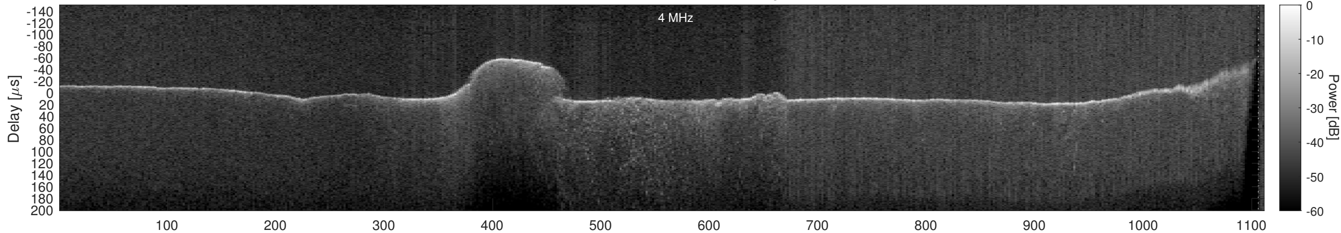
Orbit 22704, Window, Channel 1, Optimized
