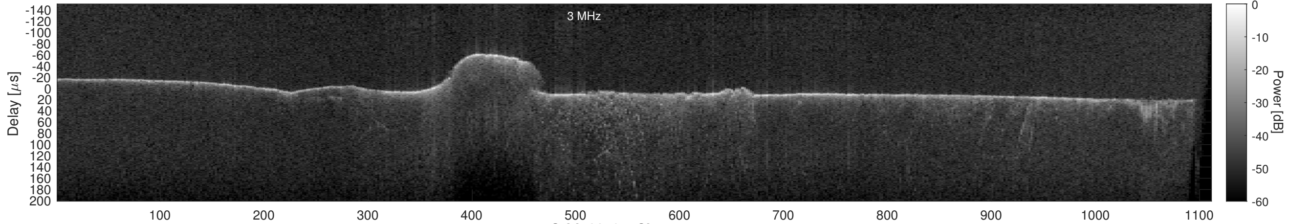
Orbit 22704, Cluttergram
