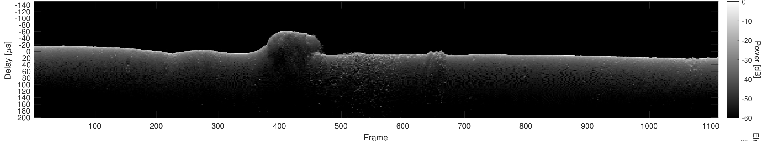
Orbit 22704, Cluttergram
