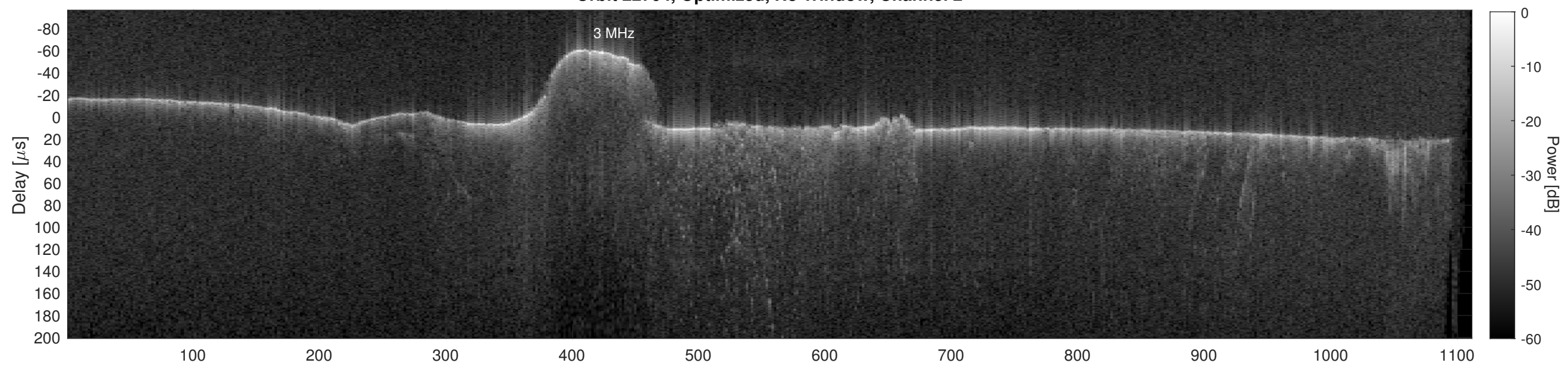
Orbit 22704, Cluttergram
