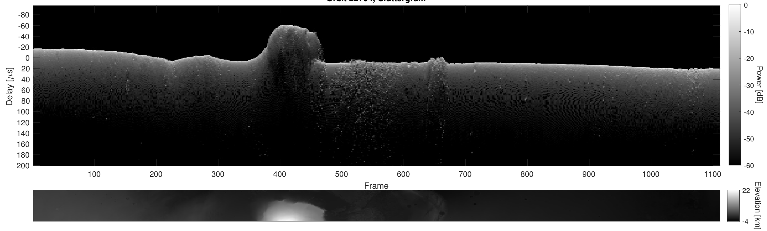
Orbit 22704, Cluttergram
