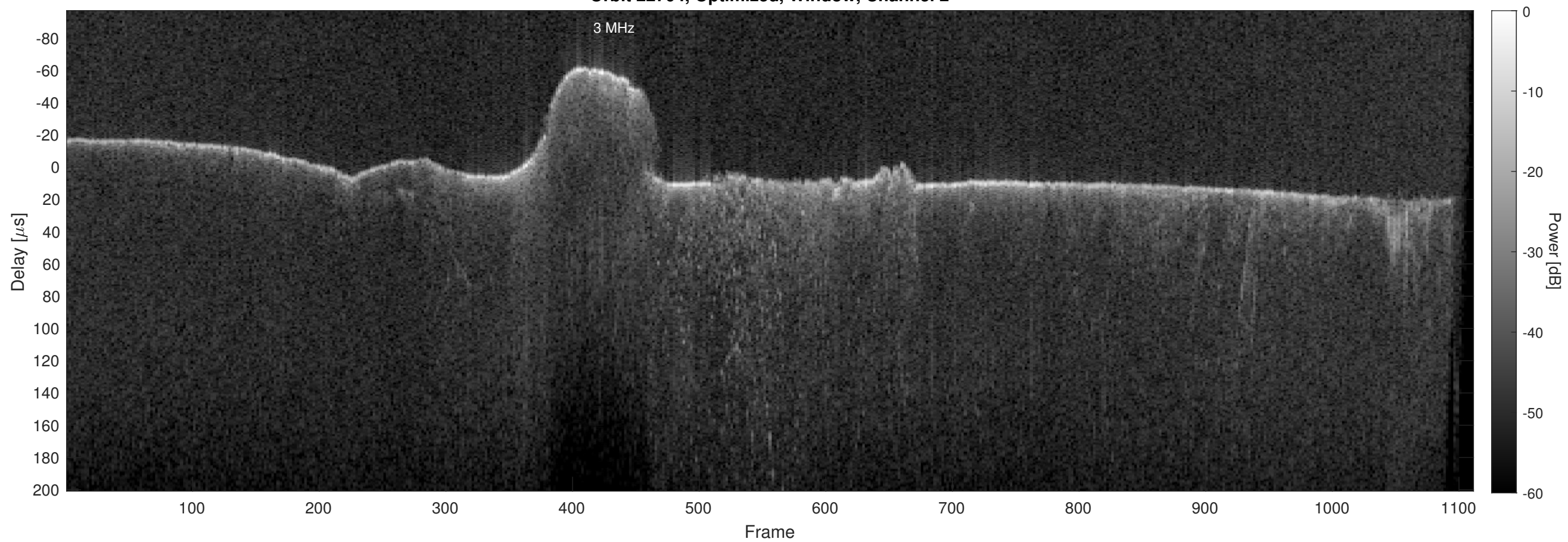
Orbit 22704, Optimized, Window, Channel 2
