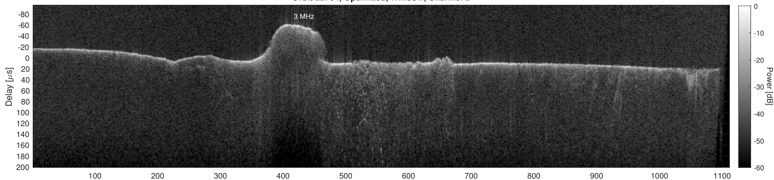
Orbit 22704, Cluttergram
