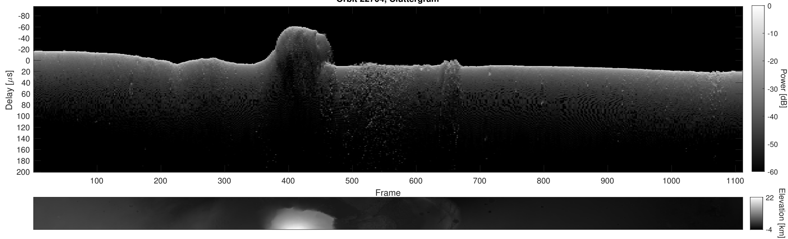
Orbit 22704, Cluttergram
