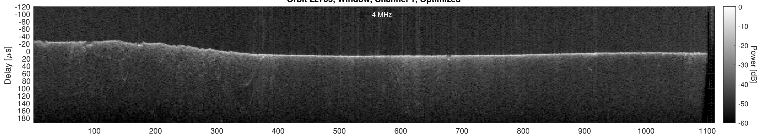
Orbit 22705, Cluttergram
