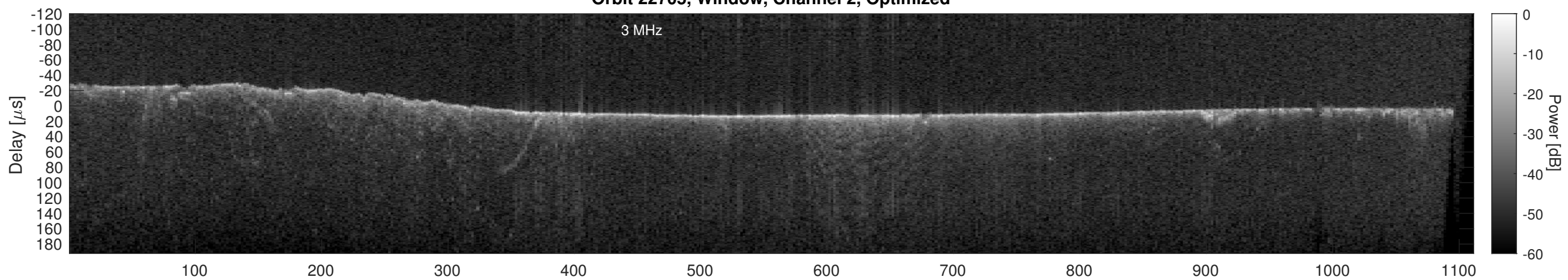
Orbit 22705, Cluttergram
