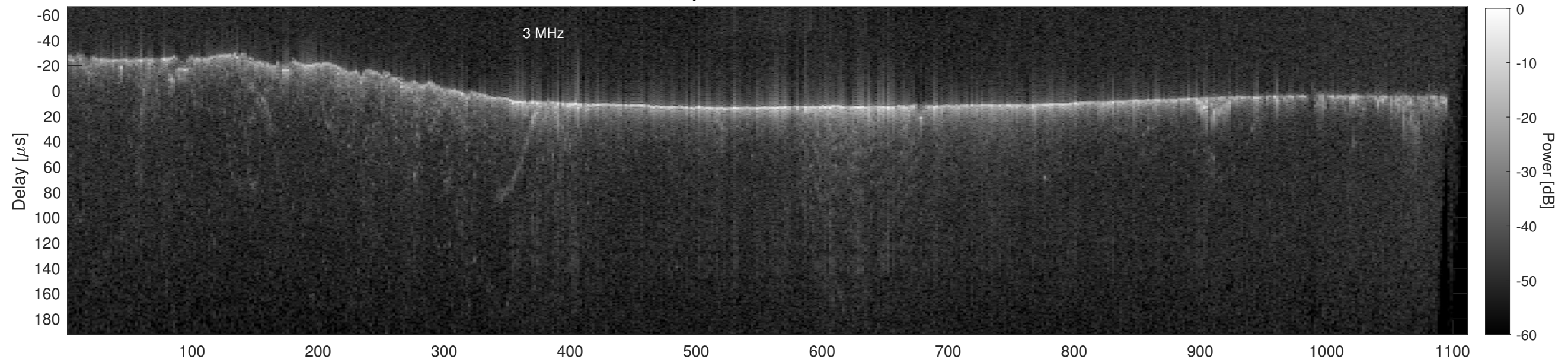
Orbit 22705, Cluttergram
