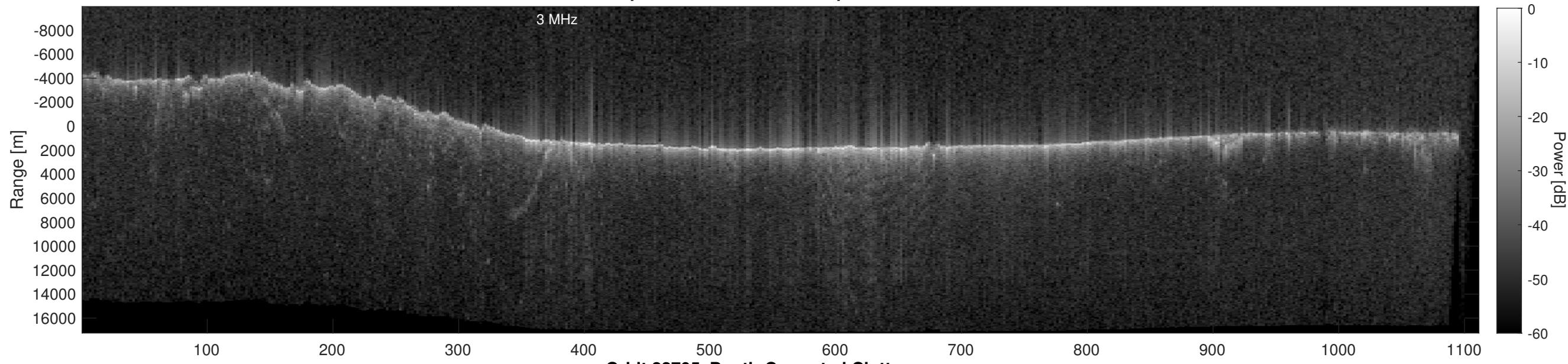
Orbit 22705, Depth-Corrected Cluttergram
