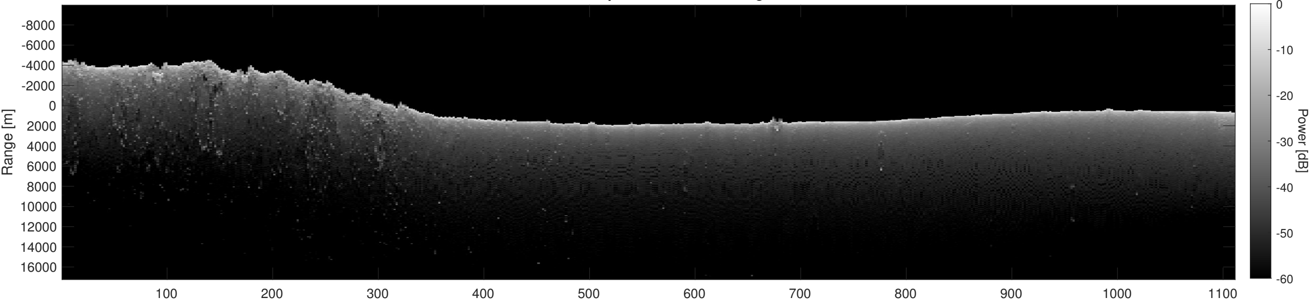
Orbit 22705, Depth-Corrected Cluttergram
