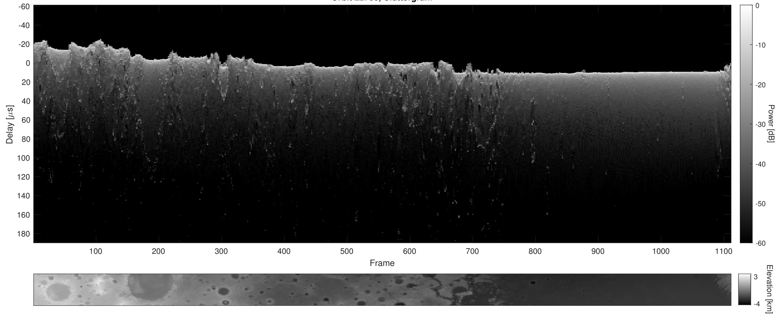
Orbit 22706, Cluttergram
