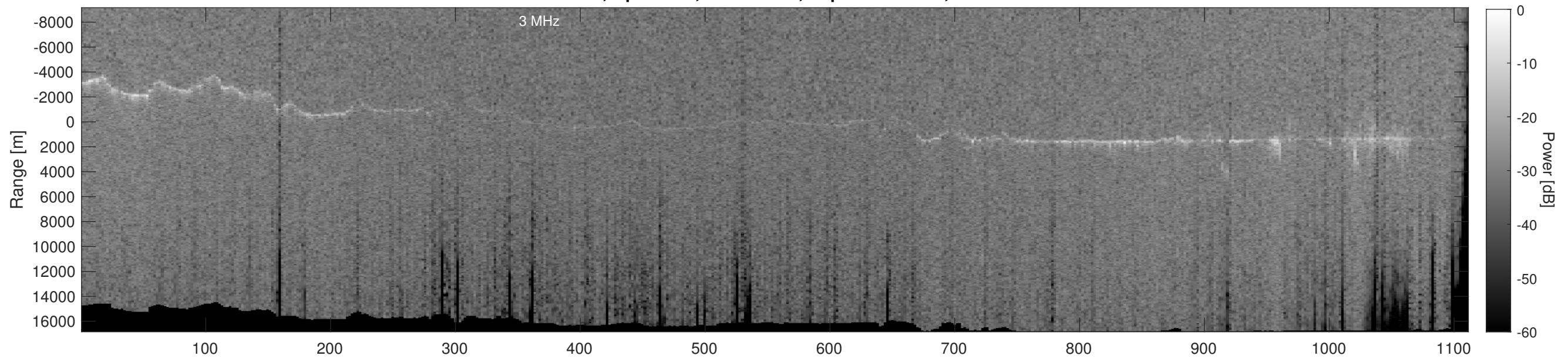
Orbit 22706, Depth-Corrected Cluttergram
