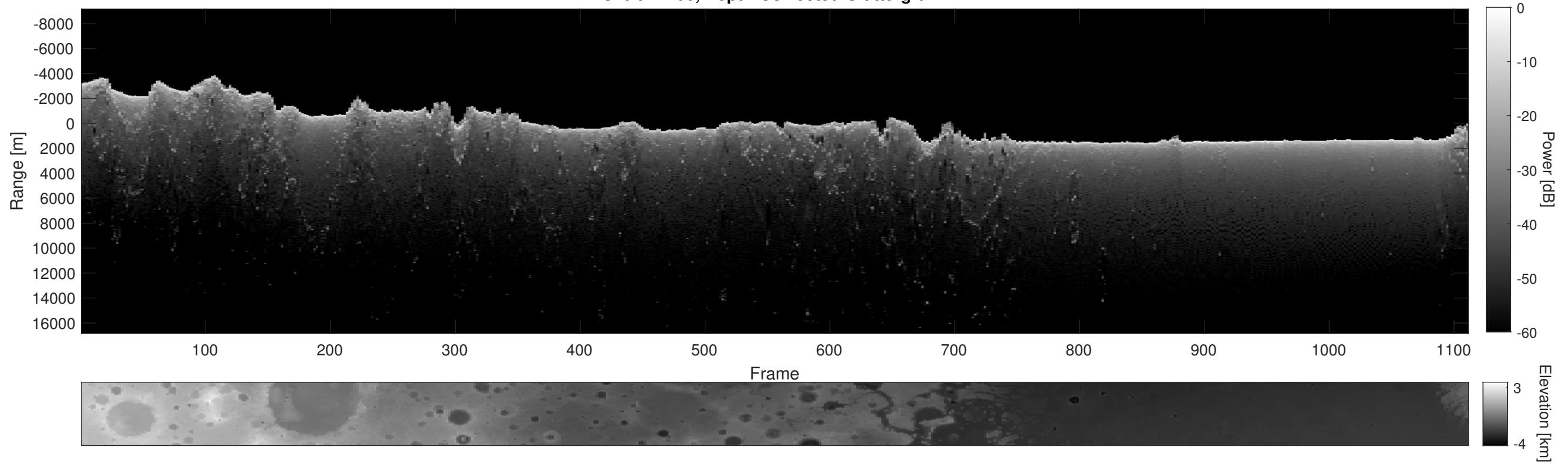
Orbit 22706, Depth-Corrected Cluttergram
