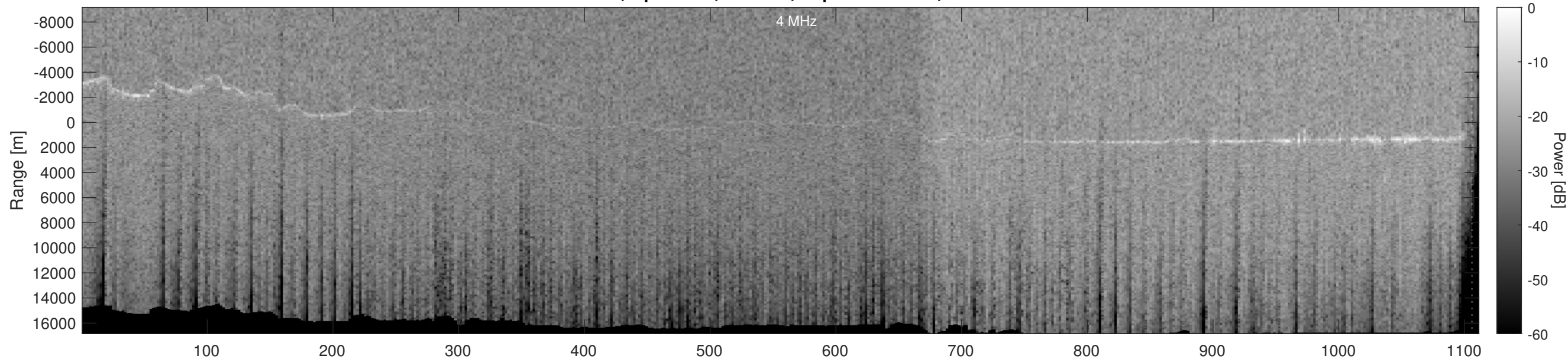
Orbit 22706, Optimized, Window, Depth-Corrected, Channel 2
