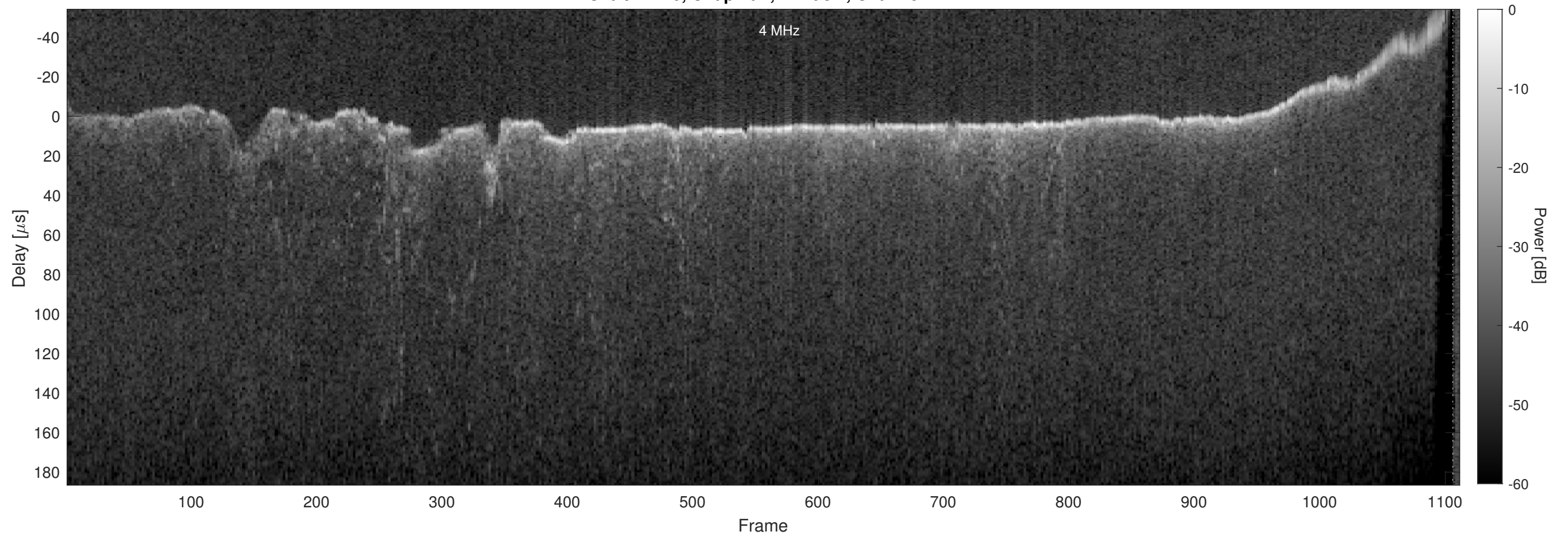
Orbit 22710, Chapman, Window, Channel 2
