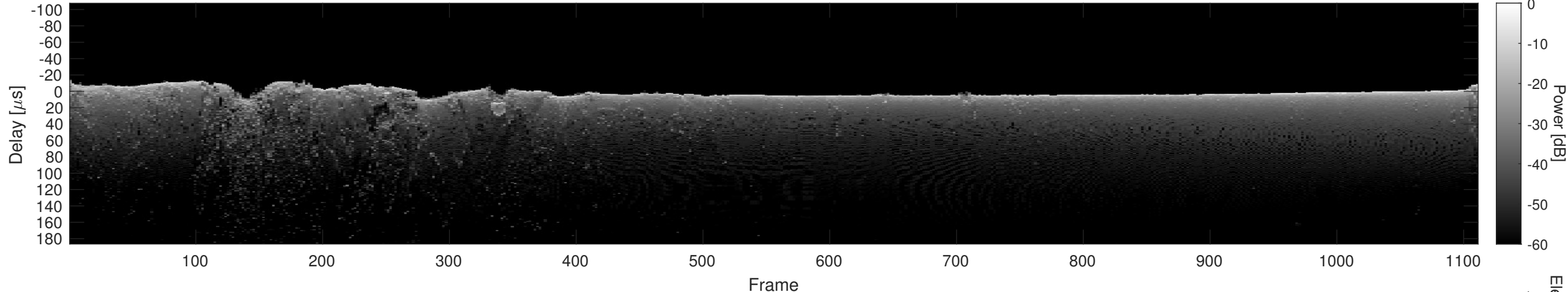
Orbit 22710, Cluttergram
