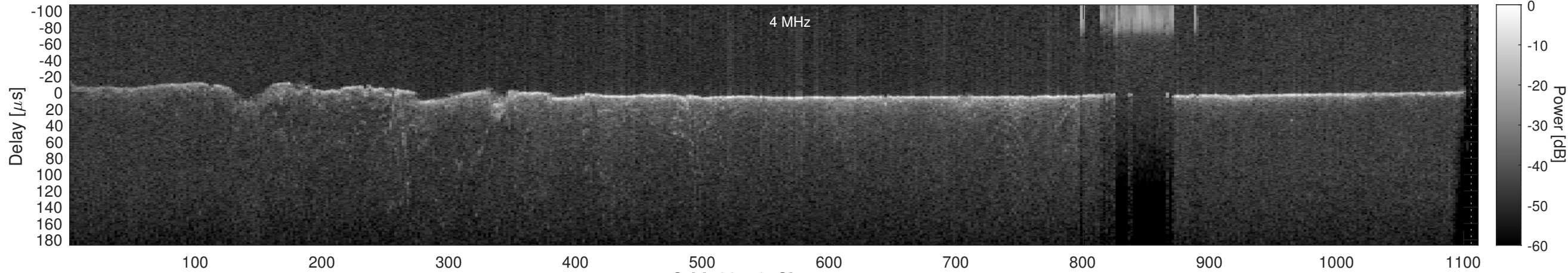
Orbit 22710, Cluttergram
