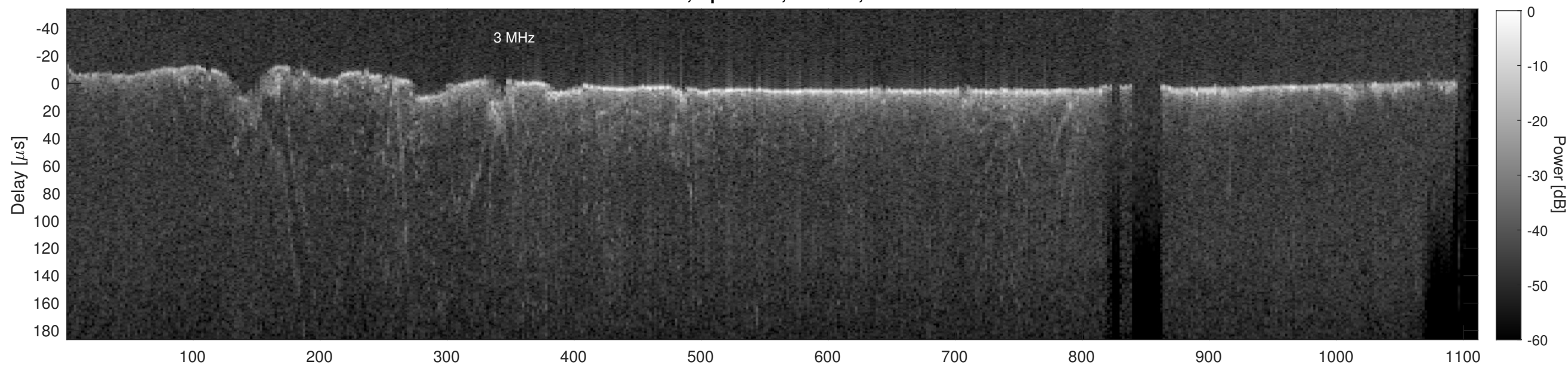
Orbit 22710, Cluttergram
